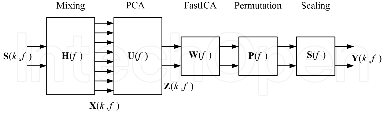
Fig. 2. The use of PCA as a pre-processing step in the frequency-domain BSS
