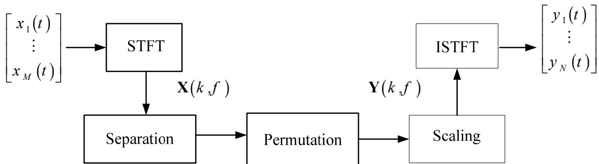
Fig. 1. System structure for the frequency-domain BSS
