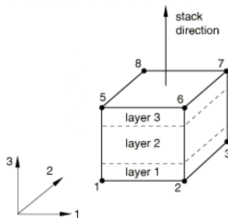
Figure 2. Solid element with composite layups
