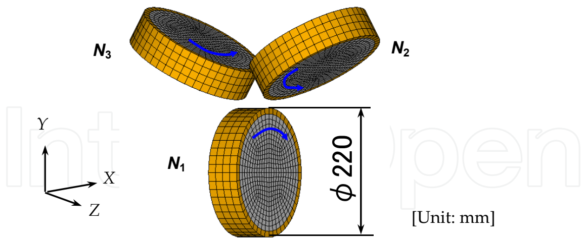
Figure 13. Finite element models of small rollers (D220).
