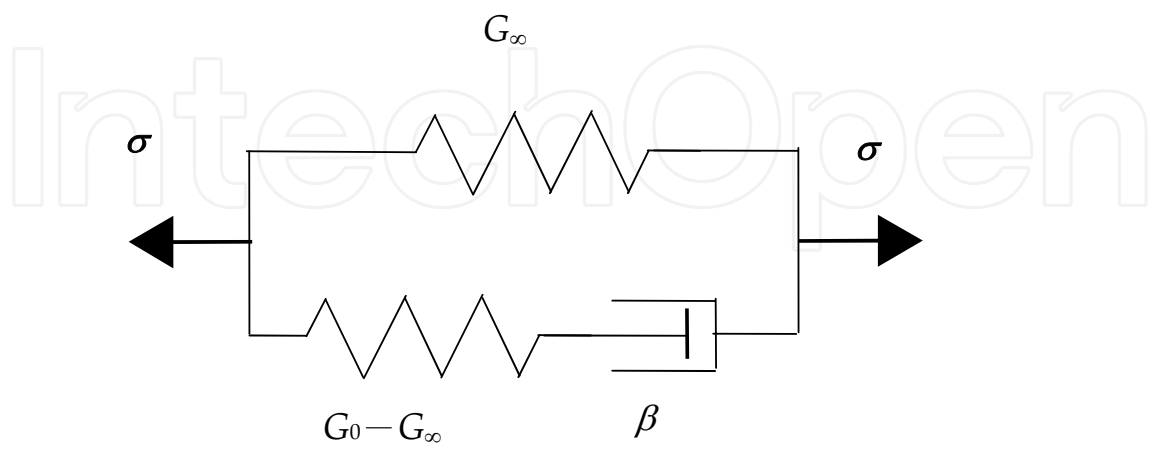
Figure 4. Viscoelastic model using three elements of the ball for baseball.
