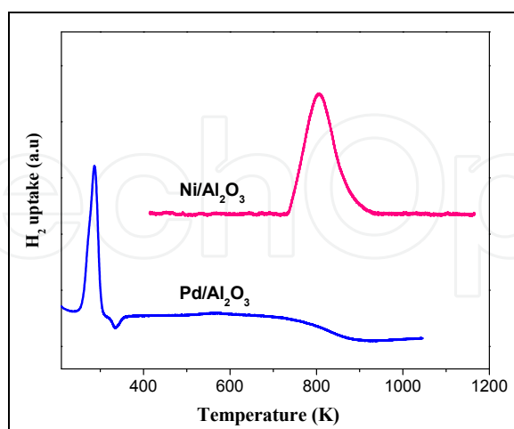
Figure 3. TPR traces of the \text{Ni/Al}_2\text{O}_3 and \text{Pd/Al}_2\text{O}_3 catalysts.
