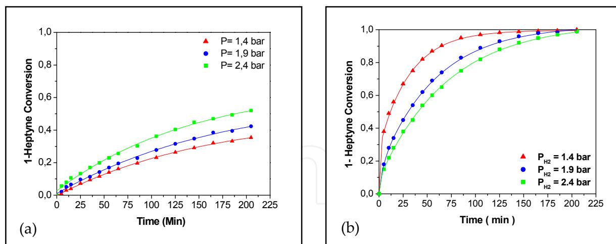
Figure 7. Effect of P_{H_2} on the catalytic activity for (a) Ni/Al 2 O 3 and (b) Pd/Al 2 O 3 . C^0_A = 0.1528 mol L -1 , T = 303 K, 800 rpm, W_{cat} = 0.3 g Ni/Al 2 O 3 or 0.03 g Pd/Al 2 O 3 , S/Ni = 64 and S/Pd = 29385 .
