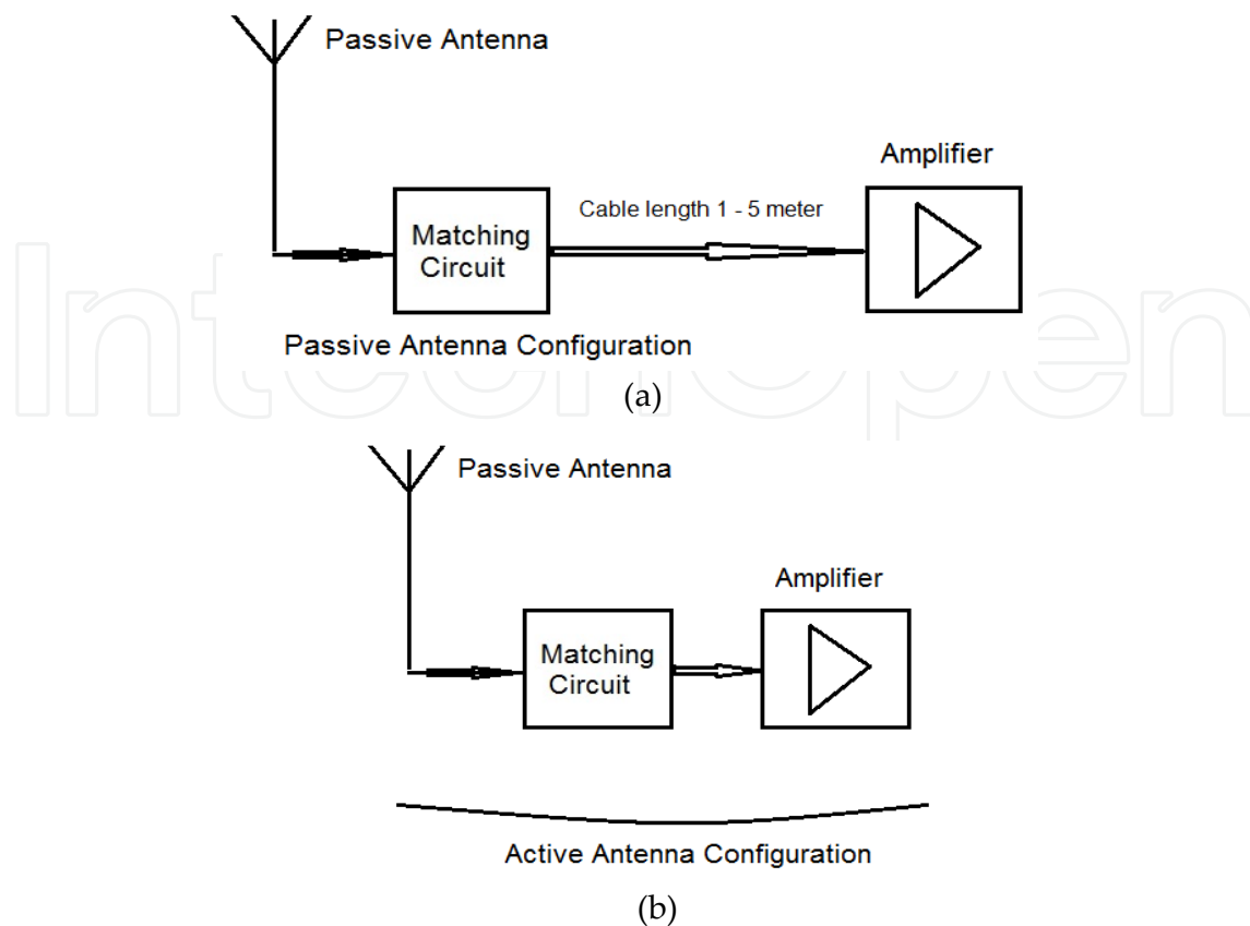
Figure 4. Passive and active antenna assembling comparison
