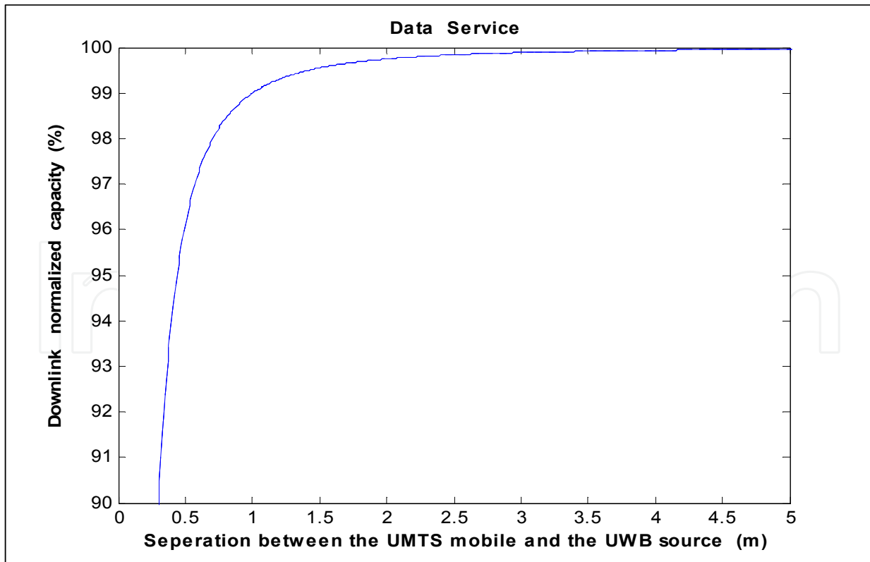
Figure 15. Effect of the UWB interference on the macrocell normalized capacity as a function of the separation between the UWB transmitter and the UMTS mobile ( P_{\text{UWB}} = -81.4 dBm/MHz).
