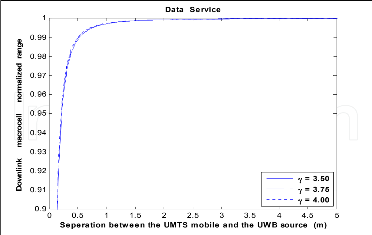
Figure 14. Effect of the UWB interference on the macrocell range as a function of the separation between the UWB transmitter and the UMTS mobile ( P_{UWB} = -81.4 \text{ dBm/MHz} ).
