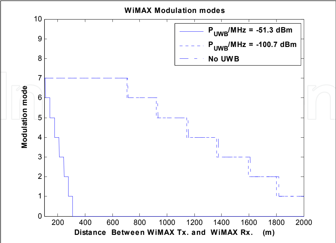
Figure 7. 2.5 GHz WiMAX modulation modes for different UWB power densities with a 1 m distance between the 4 UWB transmitters and the WiMAX receiver assuming a WiMAX transmitted power of 40 dBm/sector.
