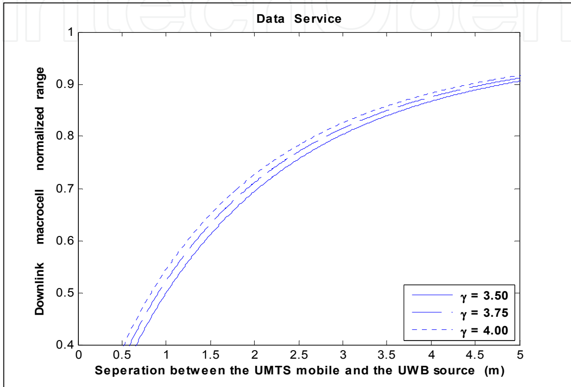
Figure 12. Effect of the UWB interference on the macrocell normalized range as a function of the separation between the UWB transmitter and the UMTS mobile ( P_{\text{UWB}} = -51.3 dBm/MHz).
