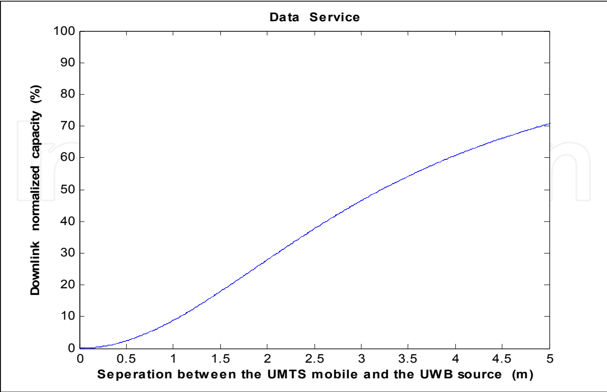
Figure 13. Effect of the UWB interference on the macrocell normalized capacity as a function of the separation between the UWB transmitter and the UMTS mobile ( P_{UWB} = -51.3 \text{ dBm/MHz} ).
