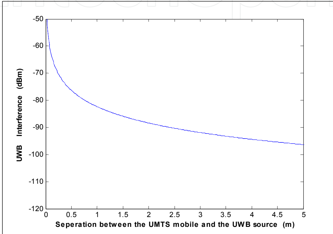
Figure 9. UWB interference as a function of the separation between the UWB transmitter and the UMTS mobile ( P_{\text{UWB}} = -51.3 dBm/MHz).
