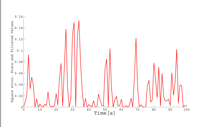
Figure 3. The square errors between the state and filtered values: 1st components
