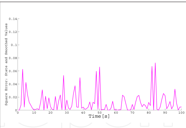
Figure 8. The square errors between the state and smoothed values: 2nd components
