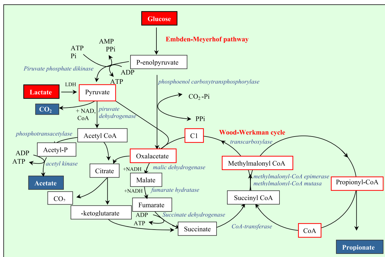
Figure 1. Propionic acid fermentation in propionibacteria
