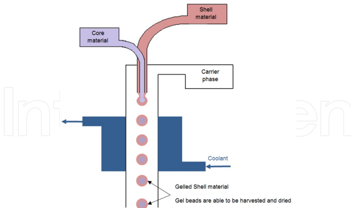
Figure 9. Schematic diagram of a submerged two-fluid static nozzle.
