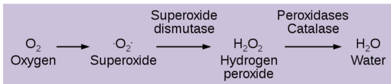
Figure 1. Enzymes involved in detoxification of O_2^{\bullet-} radical.
