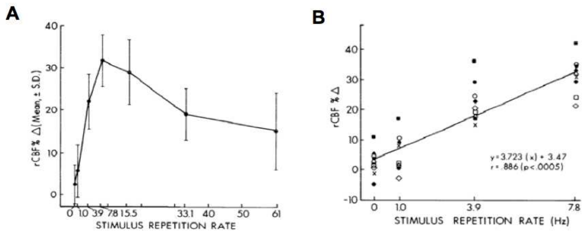
Figure 5. (A) Photoc stimulation caused a selective regional CBF (rCBF) increase in the striate cortex up to a maximum response at 7.8 Hz. The rCBF declined with frequency increases beyond 7.8 Hz but remained above the unstimulated state. Each point and error bar represent the mean \pm SD at each stimulus frequency. rCBF response is expressed as the percent change from the initial unstimulated scan. (B) Striate cortex percent change in rCBF from the initial unstimulated state, varied as a linear function of stimulus frequency between 0 and 7.8 Hz. The function of the linear regression is given and the regression line plotted. Source: (8).
