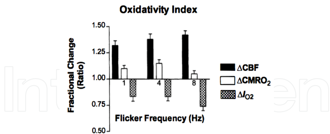
Figure 8. Percent changes of CBF, CMRO 2 , and CMRO 2 :CBF ratio index ( I O2 ) in the primary visual cortex as a function of checkerboard contrast reversal rate. Note maximum I O2 change at 8 Hz. Source: (13).
