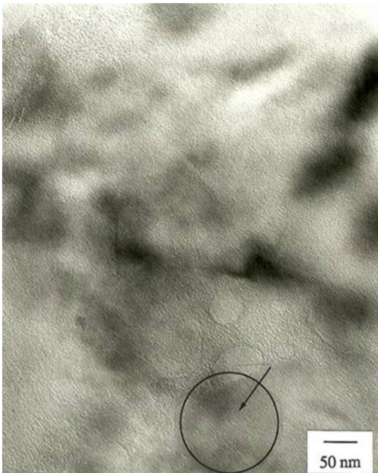
Figure 18. A and b. TEM Image of Cr 0 /CrO x -doped hexylene-bridged polysilsesquioxane under acidic condition; it reveals unusual nano-fringe patterns with alternating features of a lattice spacing of about 50 Å in different areas.
