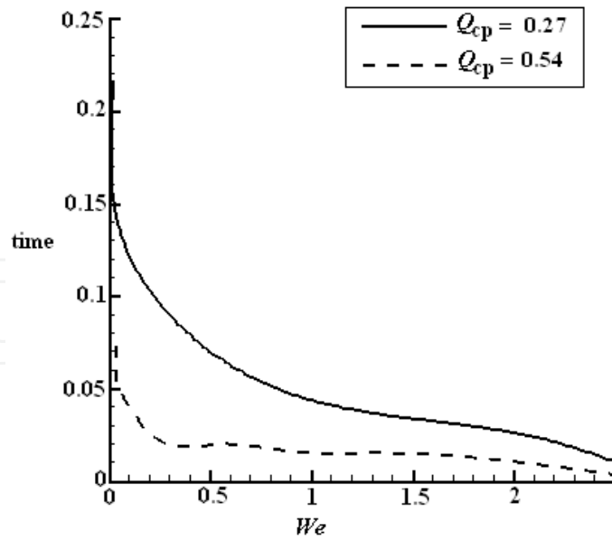
Figure 11. Detachment time of the droplet for different We number
