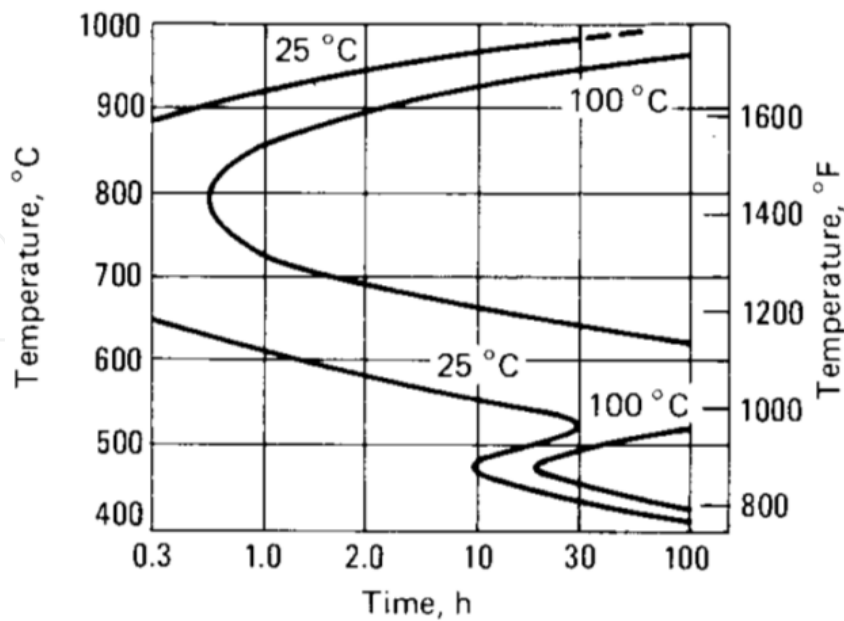
Figure 8. Time-temperature relationships to produce 25 and 100 °C DBTTs for a 29Cr-4Mo ferritic stainless steel as a function of aging times that cover both the 475 °C embrittlement range and the \sigma phase embrittlement range [24].
