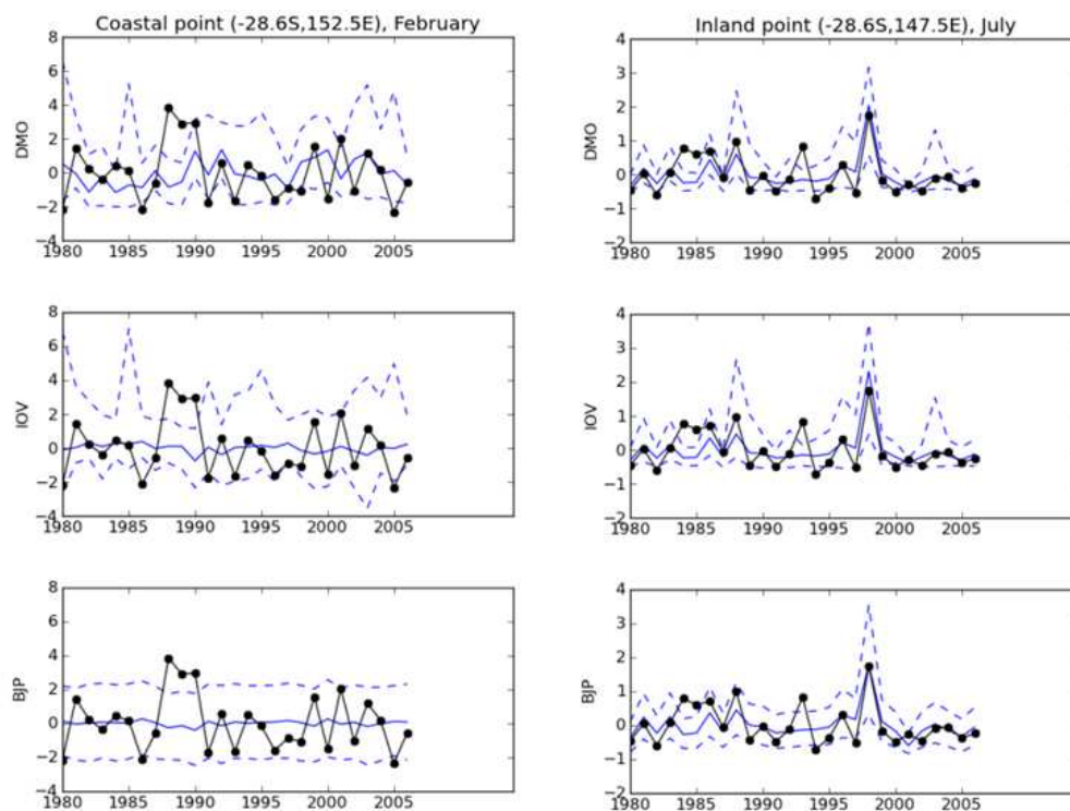
Figure 7. Effect of calibration procedures on model time series. Left: A model grid point with high hindcast correlation. Right: A model grid point with low hindcast calibration. Black line: observations, blue solid line: model mean, blue dashed line: 10% and 90% model probability intervals.
