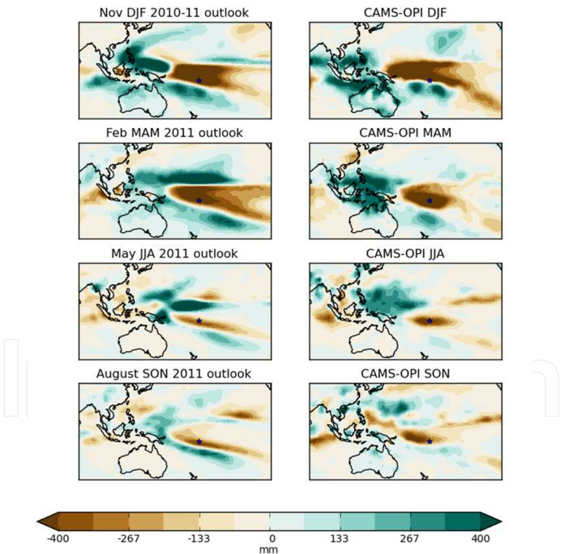
Figure 1. Left: CCGM-based predictions (left) and analysis (right) of seasonal rainfall anomalies in millimetres in the tropical South Pacific region during 2011 for the four calendar seasons starting December-January-February (DJF).
