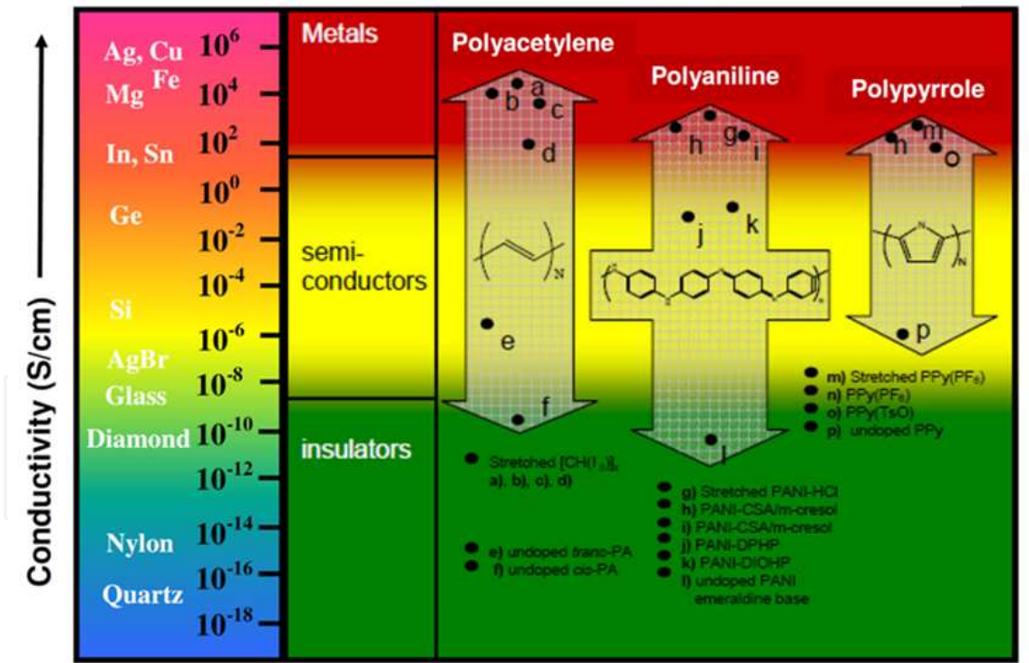
Figure 7. Conductivity of some conjugated polymers in comparison to typical metals, semiconductors or insulators.
