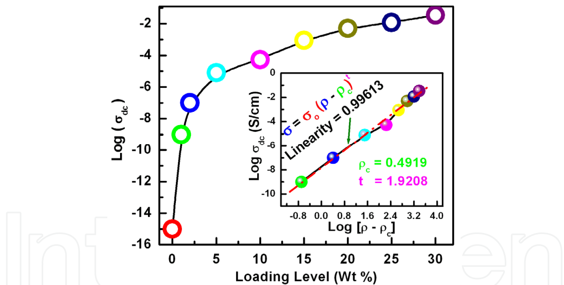
Figure 12. Variation of conductivity ( \sigma_{dc} ) of PANI-MWCNT nanofiller loaded polystyrene solution blends. Inset shows the percolation and scaling details
