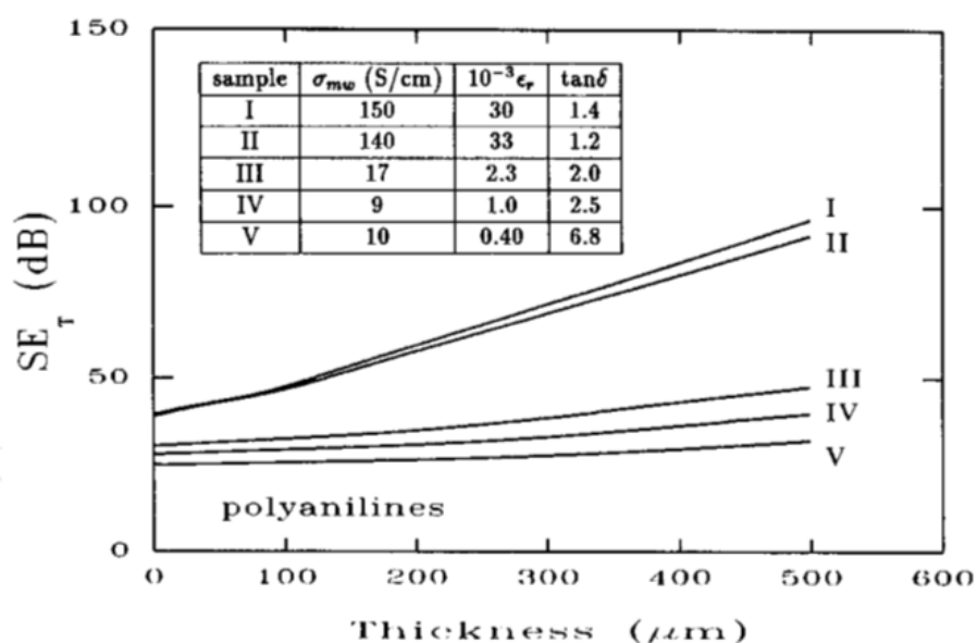
Figure 23. Thickness dependence of total shielding efficiency ( SE_r ) of various “crosslinked” polyaniline (XPANI-ES) samples. Sample I: highly XPANI-ES [3.5 times ( \times ) stretched, parallel ( \parallel )], sample II: intermediate XPANI-ES [3.5 \times , \parallel ], sample III: highly XPANI-ES (3.5 \times , \perp ), sample IV: highly XPANI-ES (unstretched), and sample V: non-XPANI-ES (12.5 \times , \perp ). Inset: comparison of \sigma_{mw} , \epsilon_r , and \tan\delta . Reprinted with permission from [J. Joo and A. J. Epstein, Appl. Phys. Lett. 65 (18), 2278-2280, 1994]. Copyright [1994], American Institute of Physics.
