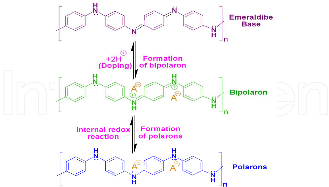
Figure 11. Protonic acid doping of polyaniline leading to formation of charge carriers polarons (radical cations) and bipolarons (dications)
