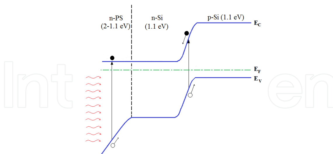
Figure 16. Energy band diagram of nPS/(n^+-p) Si solar cell.
