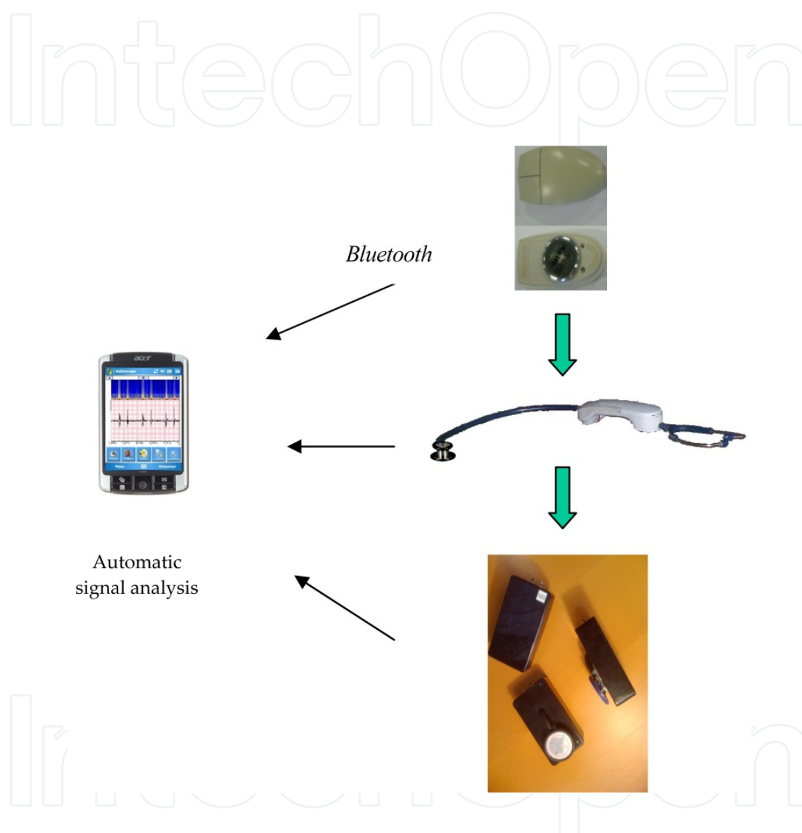
Figure 8. Several prototypes of intelligent (automatic signal analysis) communicating (Bluetooth) stethoscope system developed by our team in Strasbourg, France in different research projects, in collaboration mainly with LANNEXT, ALCATEL LUCENT, and currently with INFRAL [4].
