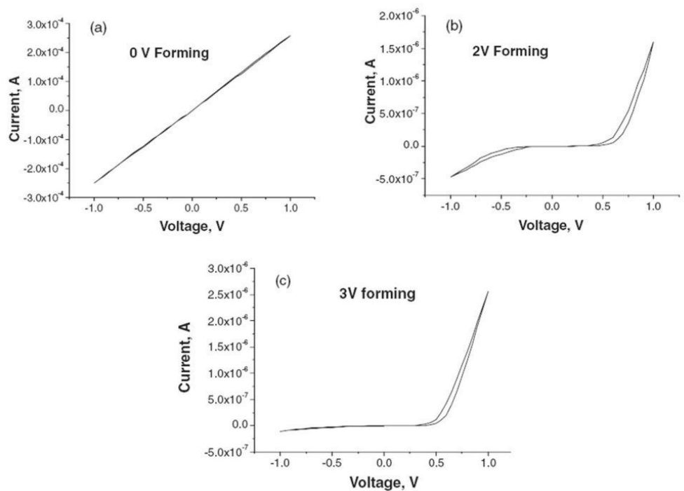
Figure 10. I-V curves of Al/GO/Al structures pre-formed at different forming voltages. (Panin et al., 2011)
