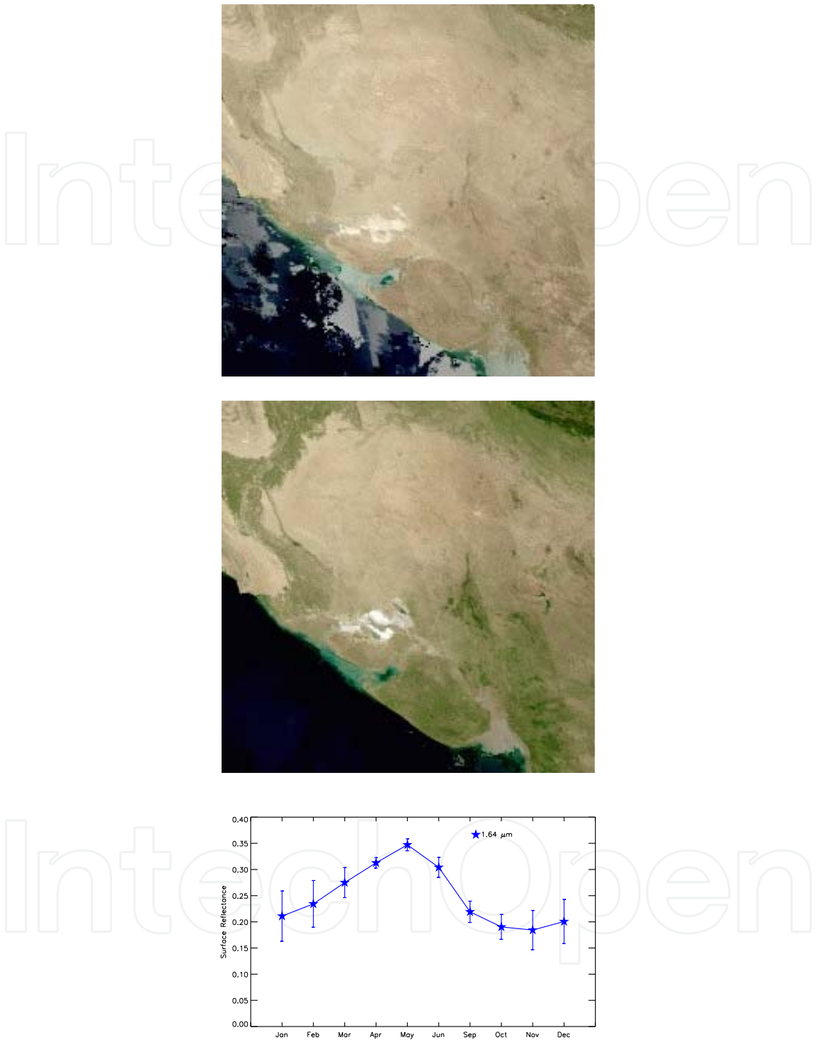
Figure 3. Picture of land surface over western India during premonsoon (top) and postmonsoon (middle) seasons, obtained from MODIS-Terra satellite. Dark black, gray and green colors represent oceanic surface, arid bare land, forest regions, respectively. (Bottom) Monthly variation of surface reflectance at 1.64 \mu\text{m} wavelength during 2007 and the vertical bars represent \pm 1\sigma deviation about the monthly mean. Note that the surface reflectance increases by 70% over study area during premonsoon.
