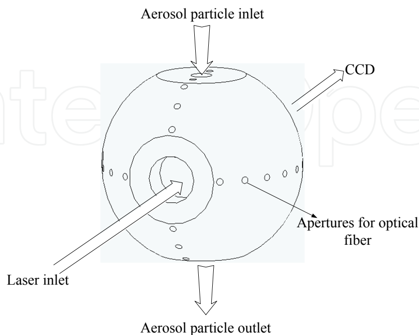
Figure 3. Simplified schematic map of aerosol particle shape and scattering analyzer
