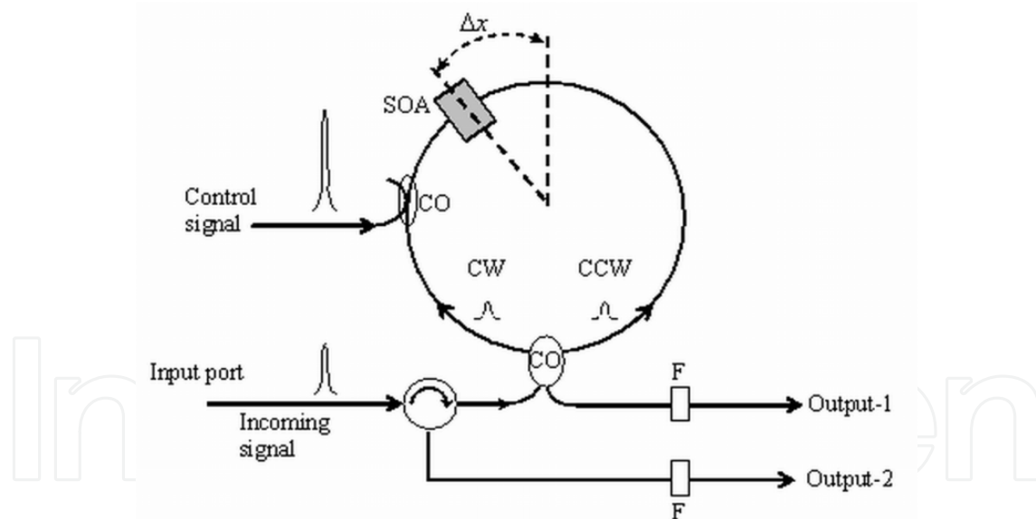
Figure 7. A TOAD based optical switch, where SOA: Semiconductor optical amplifier, CW: Clockwise pulse, CCW: Counter clockwise pulse, CO: coupler, F: Filter which blocks control pulse.
