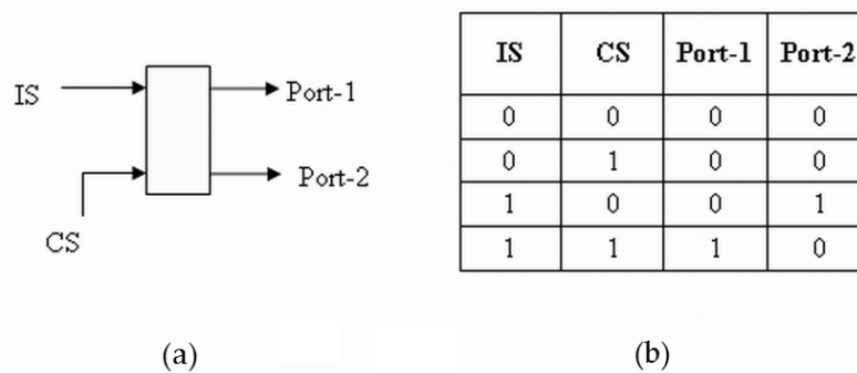
Figure 8. (a) Schematic block diagram TOAD based switch (b) the corresponding truth table.
