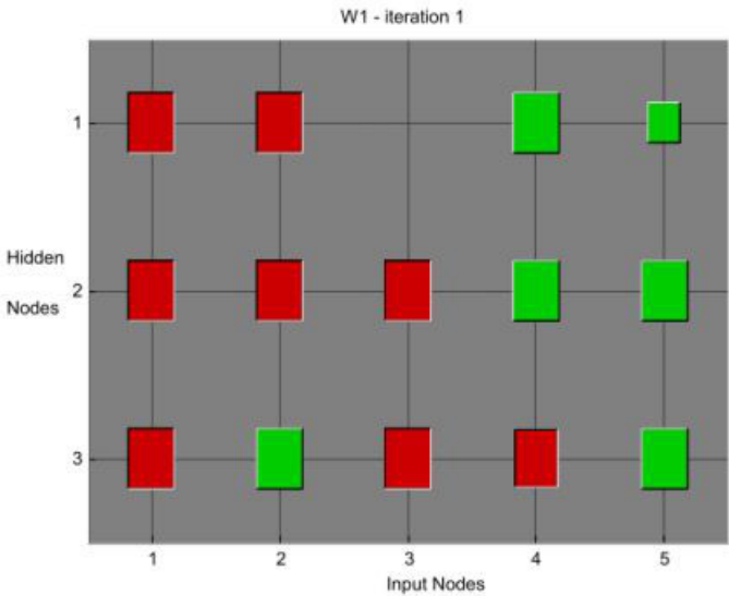
Figure 9. Hinton diagram of weight connections between input layer and hidden layer at 1st iteration.
