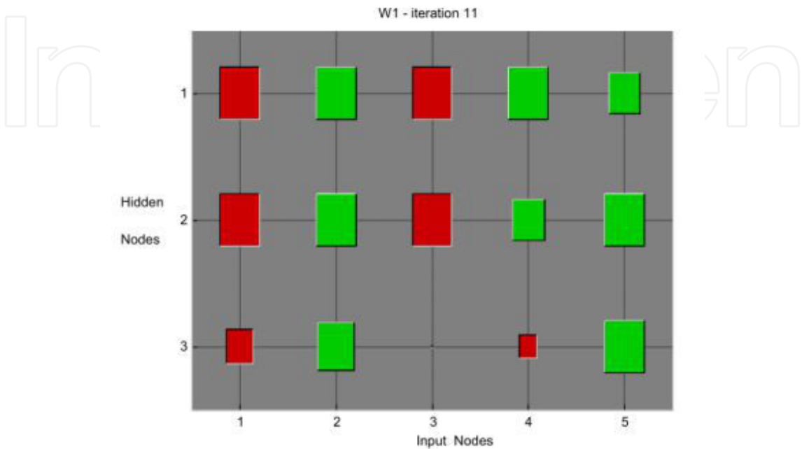
Figure 10. Hinton diagram of weight connections between input layer and hidden layer at 11th iteration.
