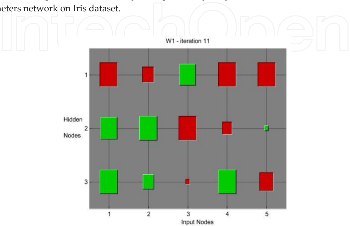
Figure 8. Hinton diagram of weight connections between input layer and hidden layer at 11th iteration.
