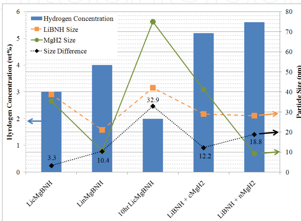
Figure 17. Comparison of hydrogen concentration and crystallite size of the quaternary LiBNH and \text{MgH}_2 phases after milling.
