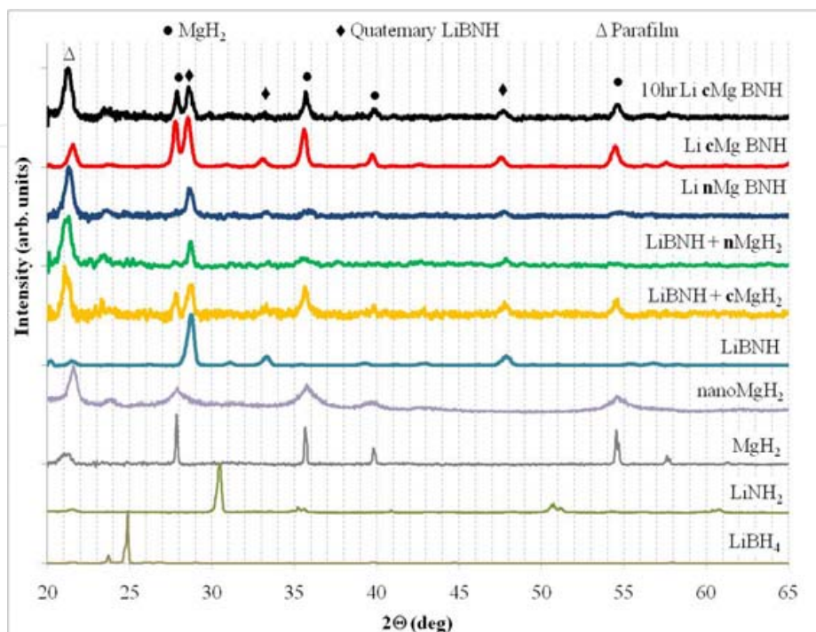
Figure 12. XRD Profile of the five differently processed materials as well as the parent compounds, LiBH 4 , LiNH 2 , MgH 2 and nano MgH 2 .
