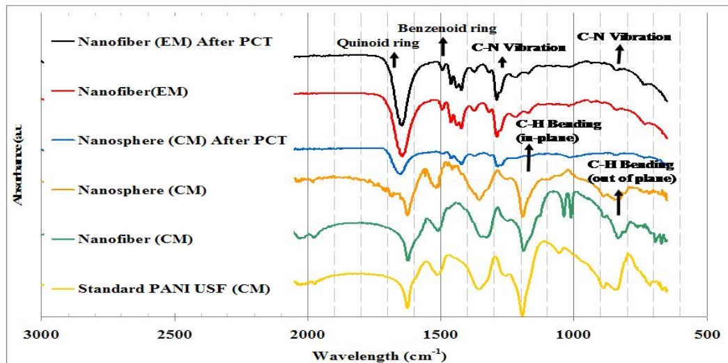
Figure 4. FTIR spectra of polyaniline nanofibers and nanospheres.
