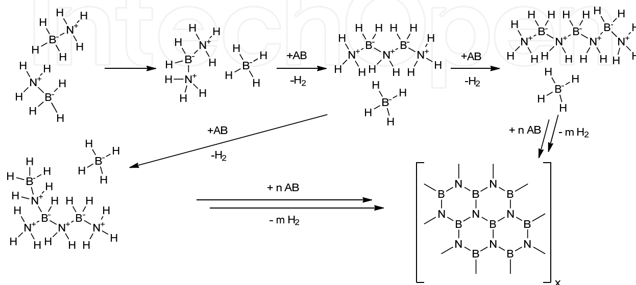
Figure 2. Decomposition Pathway of Ammonia Borane.
