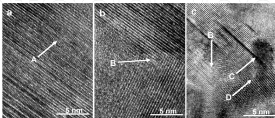
Figure 22. defects in the as-spun (30 m/s) Cu 4 alloy taken by HRTEM: (a) stacking fault, (b) twin-grain boundary, and (c) dislocations and sub-grain boundaries
