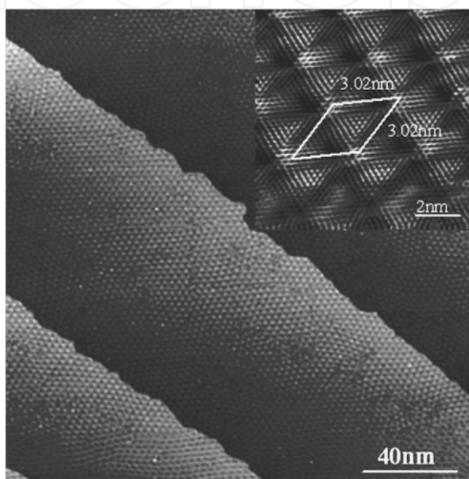
Figure 16. STM image ( 200 \text{ nm} \times 200 \text{ nm} ) of a monolayer graphene on Ru (0001). The moiré pattern with a periodicity of 30 \text{ \AA} is clearly visible. The inset shows the atomic structure of graphene/Ru (0001). The unit cell is marked as a rhombus [62].
