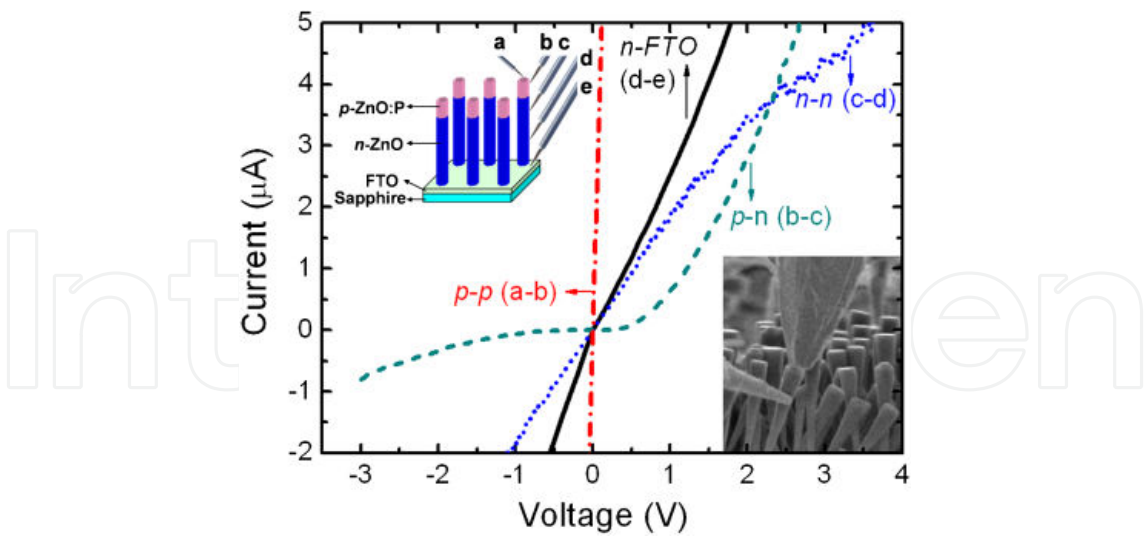
Figure 22. I – V characteristics of p – p , p – n , n – n , and n – FTO regions in a single ZnO rod. The upper left and lower right insets show the schematic diagram and a SEM image of probing by Zyrex nanomanipulator, respectively. From Ref. [97].
