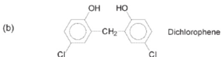
2,2'-Dihydroxy-5,5'-dichlorodiphenyl methane
