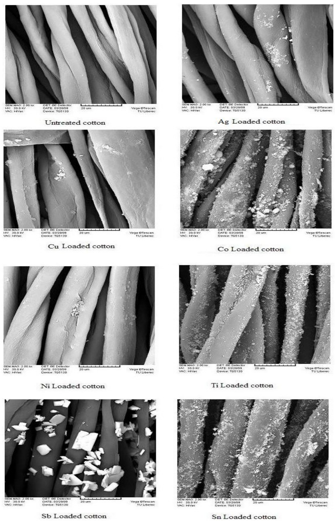
Fig. 2. The SEM images of metallic loaded cotton
