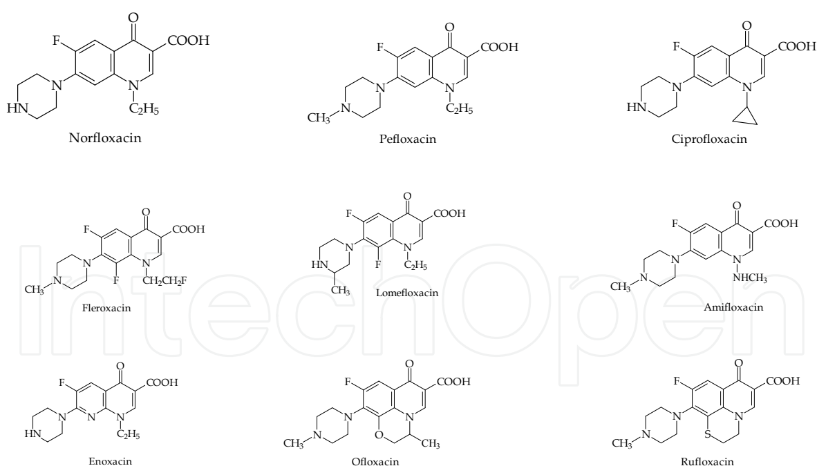
Fig. 2. Second-generation quinolones.
