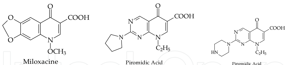
Fig. 1. First-generation quinolones.
