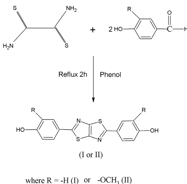
Scheme 1. Preparation of Compound I and II
