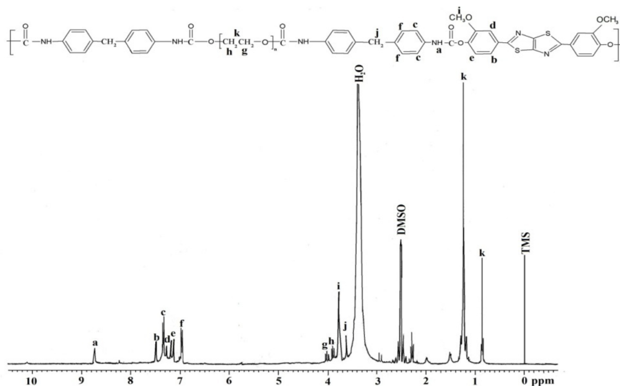
Figure 2. ^1\text{H} -NMR spectrum of LCPUE VIIa
