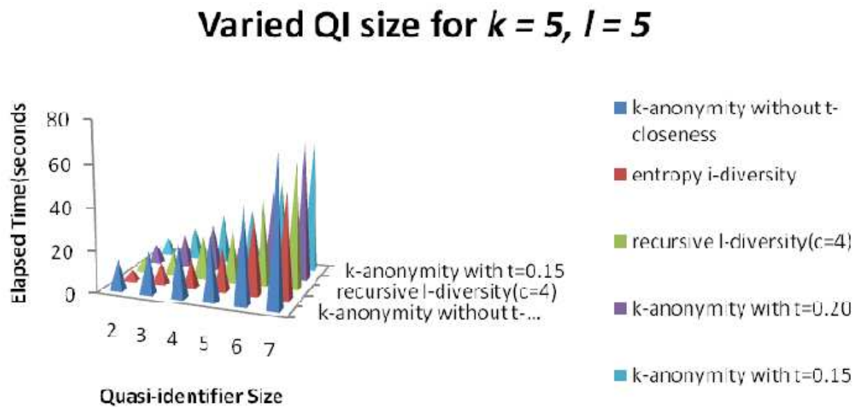
Figure 10. Elapsed time Vs. quasi-identifier size for diverse anonymity techniques
