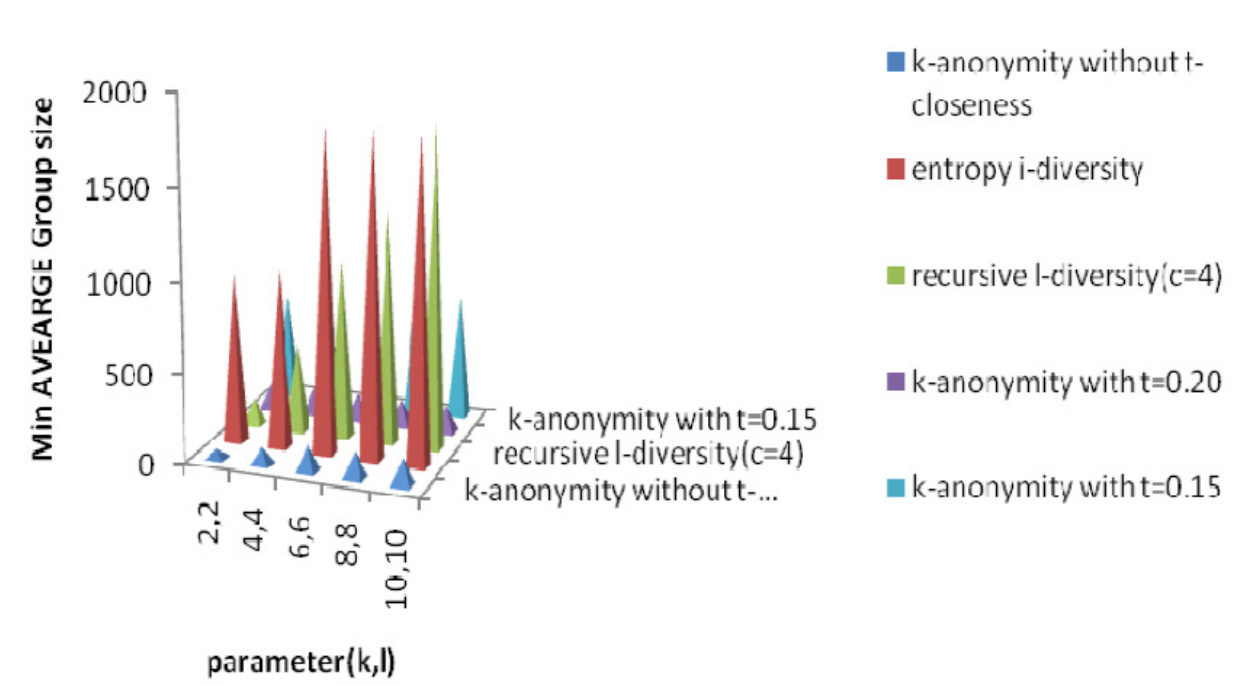
Figure 15. Minimum Average group size Versus Parameter for diverse anonymity techniques
