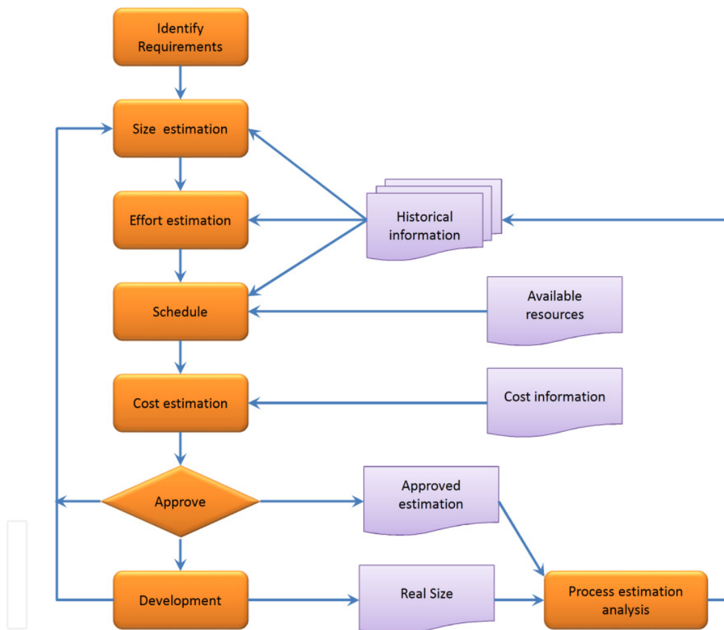
Figure 1. General stages in effort estimation.
