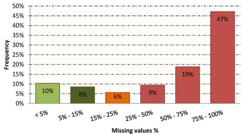
Figure 3. Frequency of missing values in dataset
