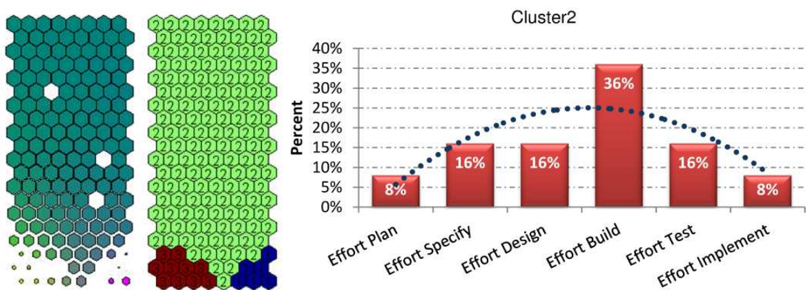
Figure 7. Identification of the load distribution of effort in the majority cluster
