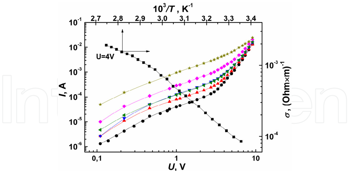
Figure 2. CVC of the structure Cr/ZnTe/Ag at various temperatures: ● – T = 298 K; ▲ – T = 303 K; ▼ – T = 308 K; ► – T = 313 K; ◆ – T = 318 K; * – T = 323 K, and the dependence \log \sigma - 1/T obtained from the ohmic section of the CVC. The film is prepared at T_e = 973 K and T_s = 823 K
