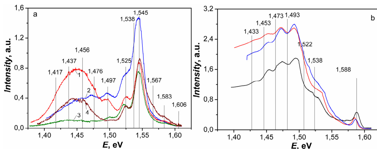
Figure 5. PL spectra registered at T = 4.5 K for polycrystalline films CdTe/glass (a), prepared at T_e = 893 K and various T_s , K: 473 K (1); 523 K (2); 623 K (3); 823 K (4) and for the epitaxial layer CdTe/BaF 2 (b): T_e = 893 K, T_s = 798 K
