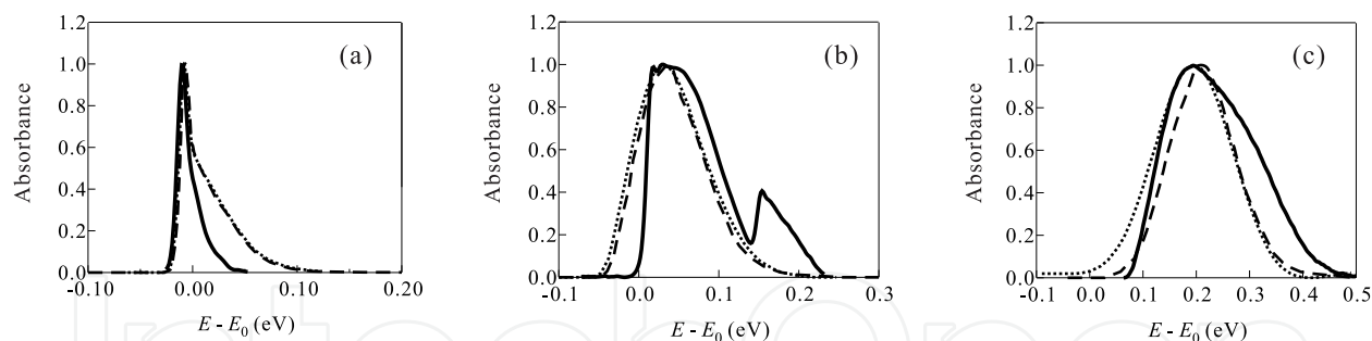
Figure 5. The line shape simulation of the \text{CH}_3\text{I} 6s transition doped into supercritical argon using (---) a semi-classical line shape function data [33] and using ( \cdots ) molecular dynamics [32] in comparison to (—) the photoabsorption spectra at (a) \rho_{\text{Ar}} = 2.0 \times 10^{21} \text{ cm}^{-3} , (b) \rho_{\text{Ar}} = 7.6 \times 10^{21} \text{ cm}^{-3} , and (c) \rho_{\text{Ar}} = 2.0 \times 10^{22} \text{ cm}^{-3} . Experimental data are from the present work.
