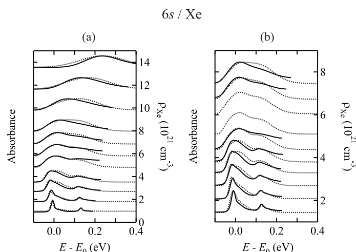
Figure 13. Selected photoabsorption spectra (—, relative units) and simulated line shapes ( \cdots ) for the CH 3 I 6s Rydberg transition in xenon at (a) non-critical temperatures and (b) on an isotherm ( 17.0^\circ\text{C} ) near the critical isotherm. The data are offset vertically by the xenon number density \rho_{\text{Xe}} . The transition energy is E_0 = 6.154 eV for the unperturbed CH 3 I 6s Rydberg transition. The variation between experiment and simulation is caused by other vibrational transitions and by perturber-dependent lifetime broadening not modeled here.
