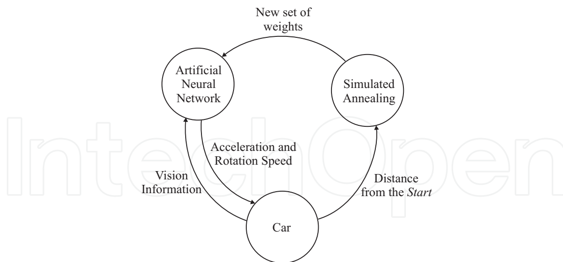
Figure 1. System architecture.
