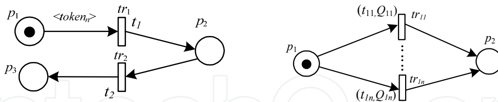
Figure 2. Transformation from high-level Petri net to the learning model
