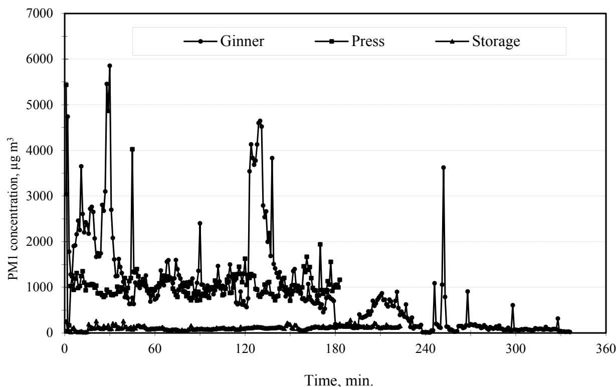
Figure 9. Continuous PM1.0 concentration measurements in three different working areas of ginner (Arslan and Aybek, 2011)
