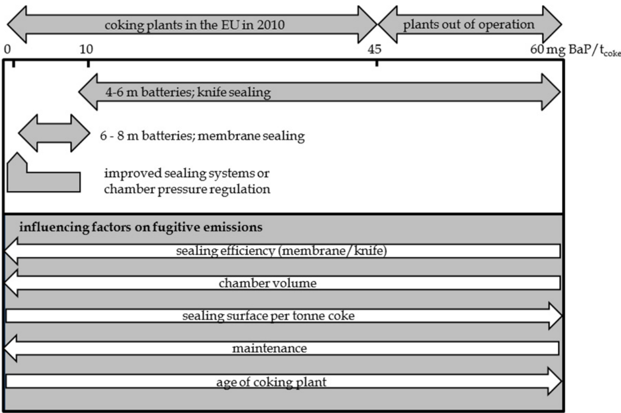
Figure 28. Typical ranges for Benzo(a)pyrene emissions (mg BaP/t coke ) from single leaks at coke oven doors as received from measurements
