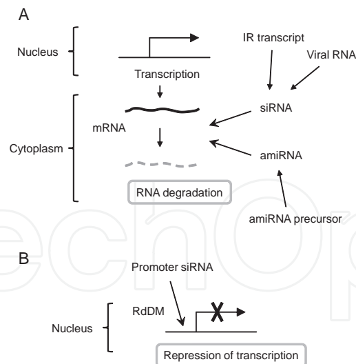
Figure 4. Various pathways of RNA silencing that can be intentionally induced to suppress gene expression in plants. Transcripts from transgenes that have an IR sequence of a plant gene segment or viral genomic RNA that carries the segment can form dsRNA. These dsRNAs are subsequently processed into siRNAs in the cytoplasm. Similarly, amiRNA precursors transcribed from the amiRNA gene are processed into amiRNAs. These small RNAs can cause degradation of target gene transcripts, a process termed PTGS (A). When siRNAs corresponding to a gene promoter are produced, they can induce RdDM in the nucleus, thereby TGS of the target gene can be induced (B). Abbreviations: amiRNA, artificial microRNA; PTGS, posttranscriptional gene silencing; RdDM, RNA-directed DNA methylation; TGS, transcriptional gene silencing.
