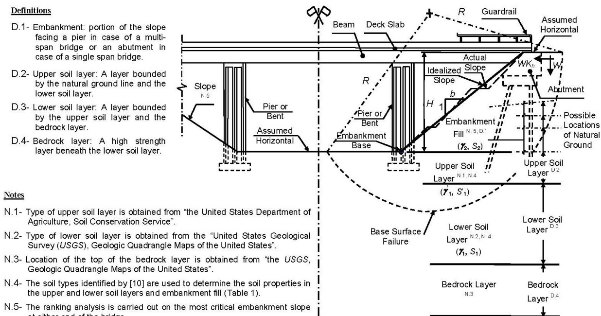
Figure 1. Bridge embankment representation for seismic ranking
