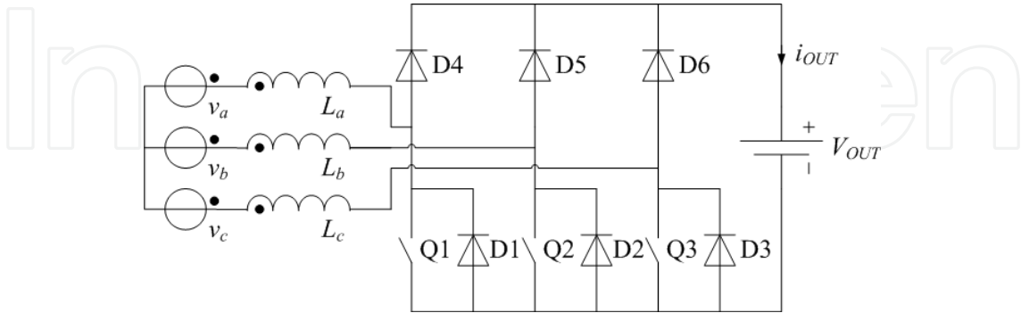
Figure 20. Boost semi-bridge rectifier (BSBR)
