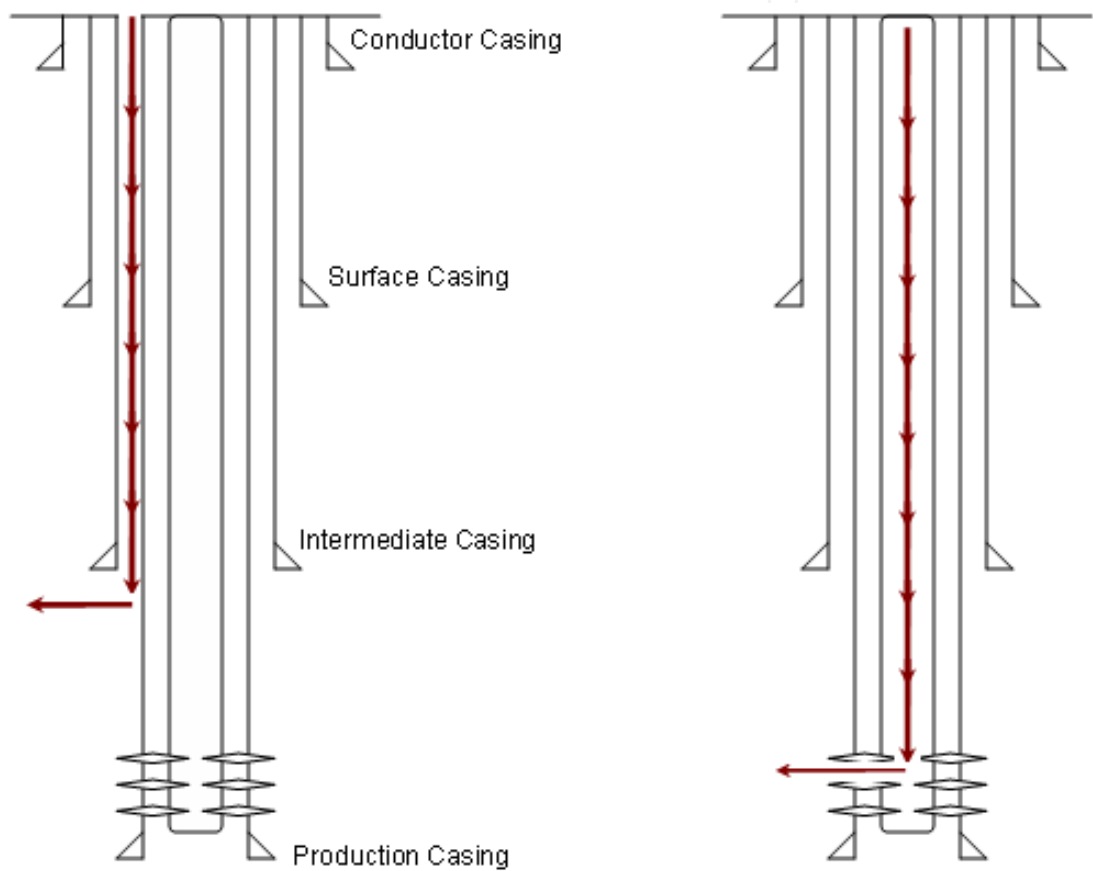
Figure 8. Two major types of DCRI; annulus injection (left) and dedicated well (right).
