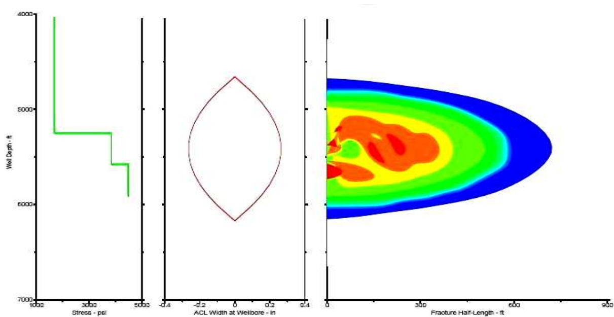
Figure 11. Fracture profile and cuttings concentration- Radial model (Case 2).
