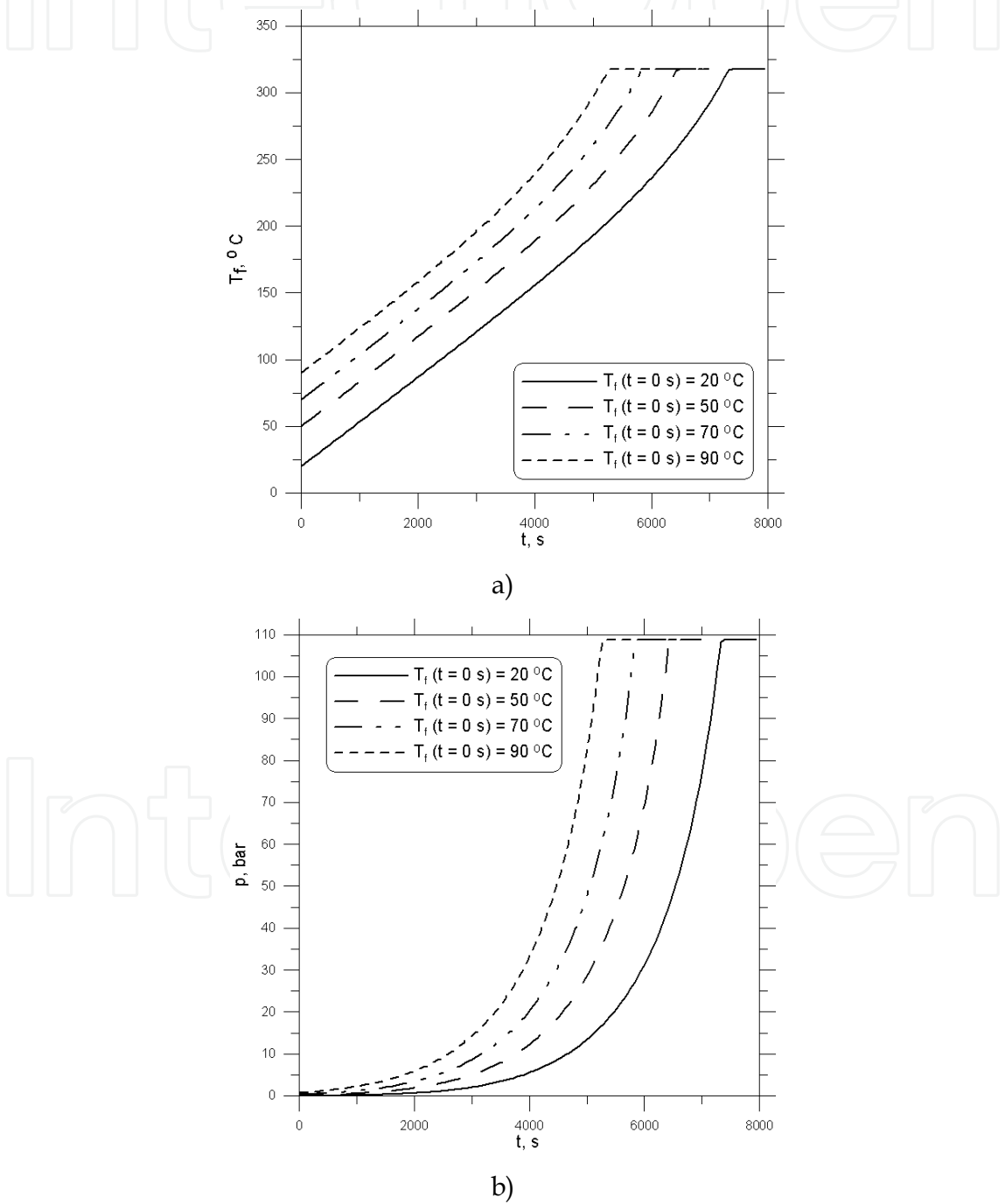
Fig. 13. Temperature and pressure of the water in the drum during boiler start-up.
