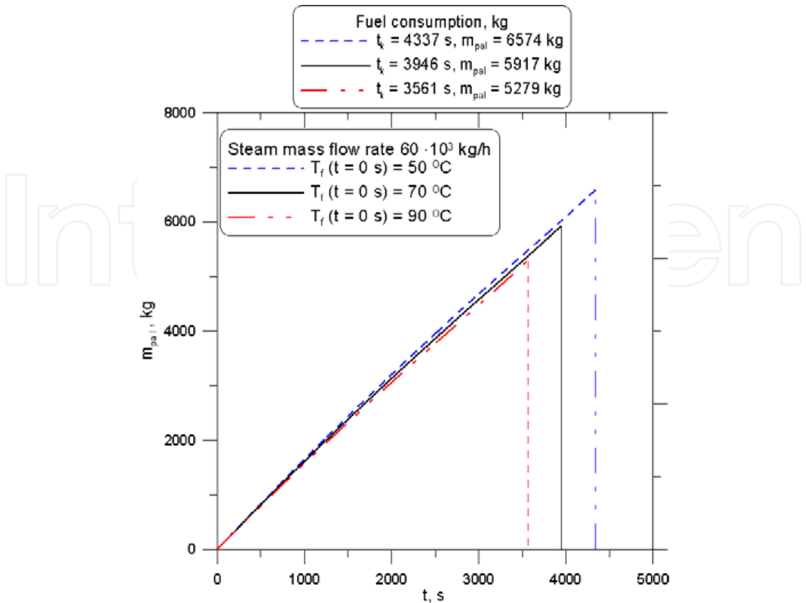
Fig. 14. Fuel consumption and boiler start-up time at different initial jumping changes in water temperature in the evaporator boiler. An analysis of the results in Fig. 14 shows that the release of the initial jump in the temperature of the boiler start-up reduces the time and reduces fuel consumption.
