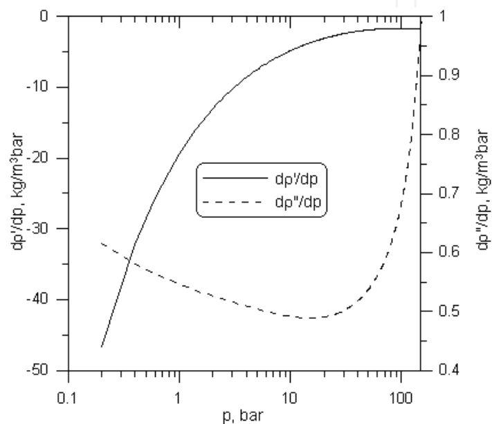
Fig. 5. Changes of the dp'/dp and dp''/dp derivatives as a function of pressure.
