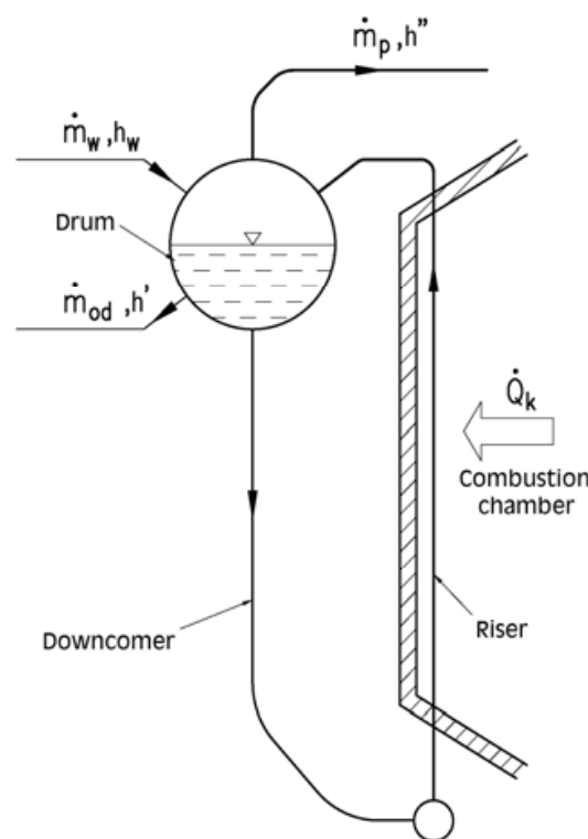
Fig. 4. Diagram of the boiler evaporator.
