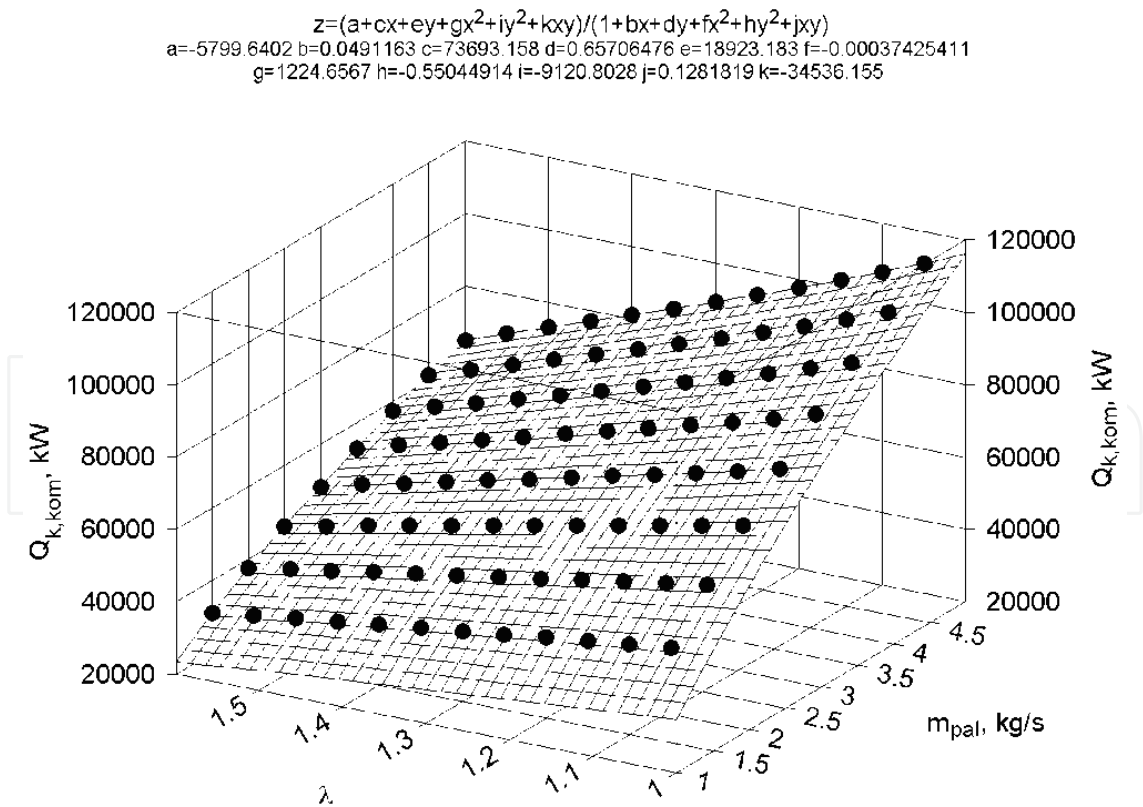
Fig. 7. Heat flow rate \dot{Q}_{k, kom} , in kW, delivered to the evaporator of the OP-210M boiler, as a function of the fuel mass flow rate \dot{m}_{pal} in kg/s and the air excess coefficient \lambda .
