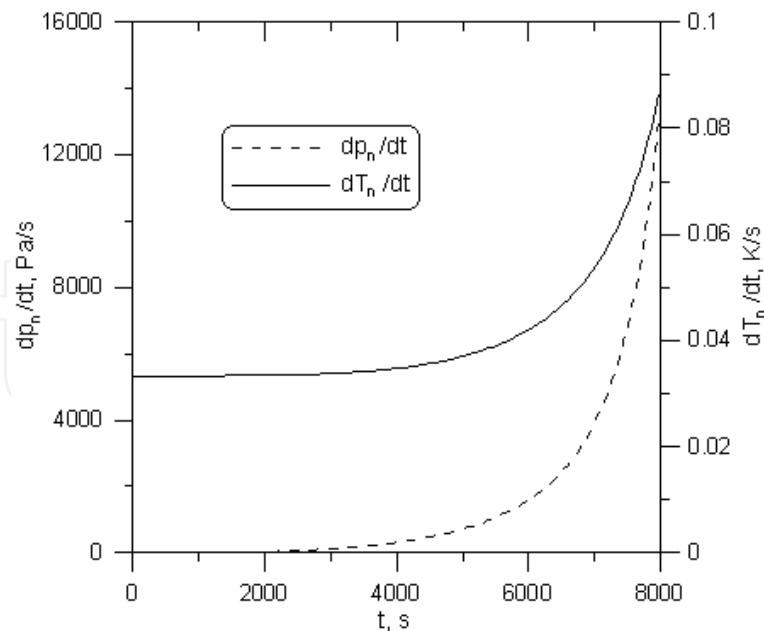
Fig. 2. Temperature and saturation pressure changes in the boiler evaporator during the heating process. After determining the T_n(t) and dT_n/dt time run, it is possible to determine the rate of pressure changes dp_n/dt using the following formula:
