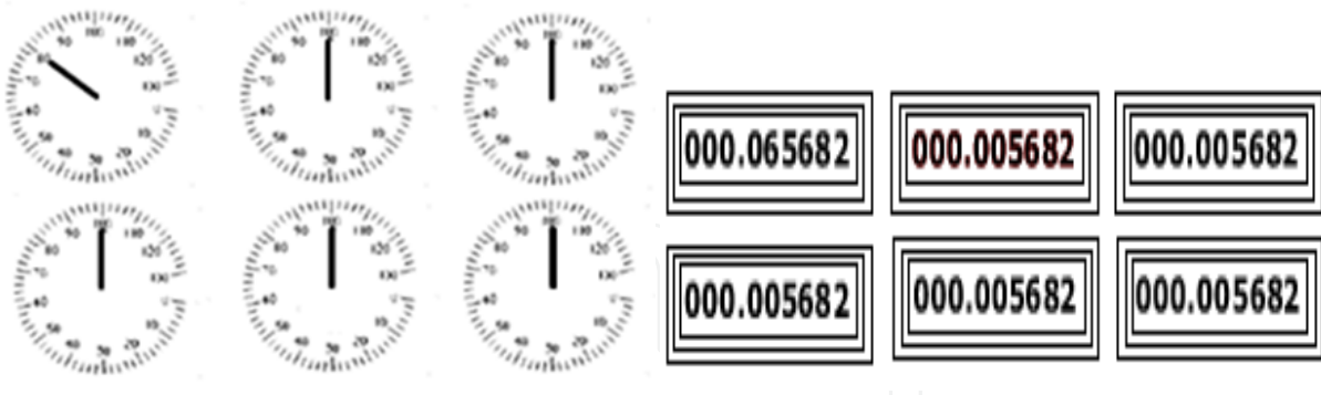
Disrupted symmetry
