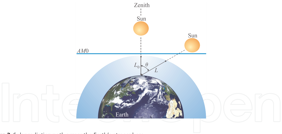
Figure 3. Solar radiation path across the Earth's atmosphere.
