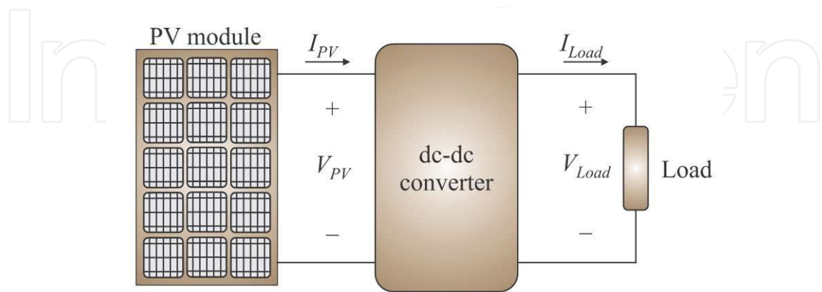
Figure 11. Maximum point tracker system.
