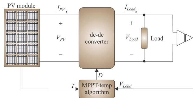
Figure 21. Configuration of the new tracking method.
