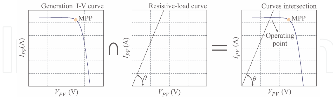
Figure 9. Definition of the system operating point by the I-V and load curves intersection.
