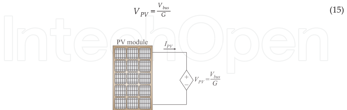
Figure 18. Equivalent MPPT system obtained from the PV module terminals.
