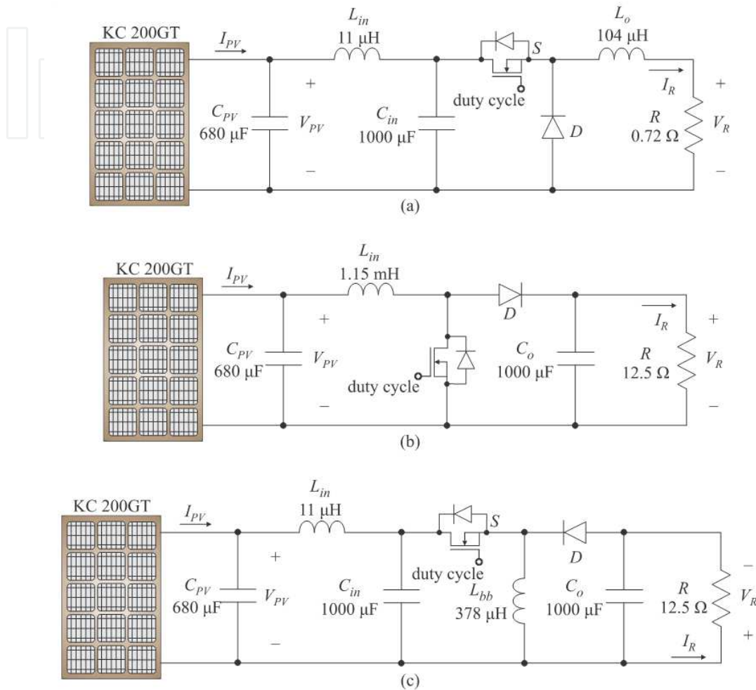
Figure 15. a) buck, (b) boost and (c) buck-boost power stage converters.
