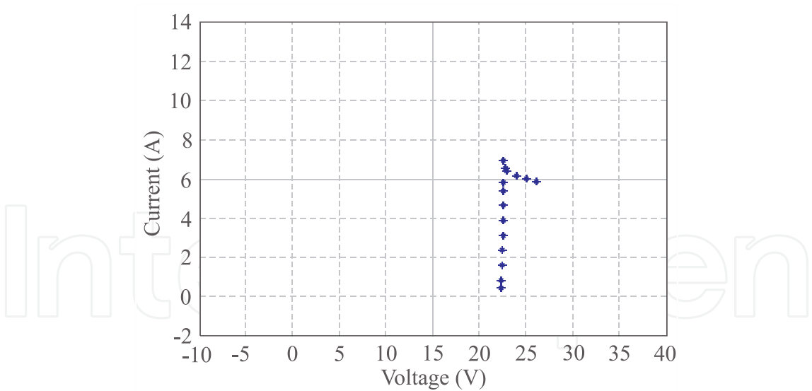
Figure 23. Theoretical MPP trajectory for solar radiation and temperature measured during experimental evaluation.
