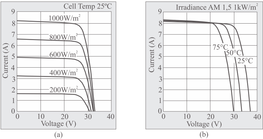
Figure 4. I-V curve from Kyocera KC200GT PV module: (a) under constant temperature and (b) under constant irradiance.
