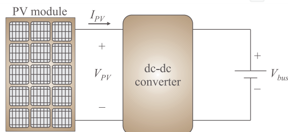
Figure 17. MPPT supplying a constant voltage load-type.
