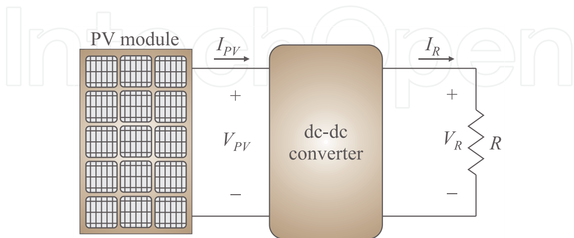
Figure 12. MPPT supplying a resistive load-type.
