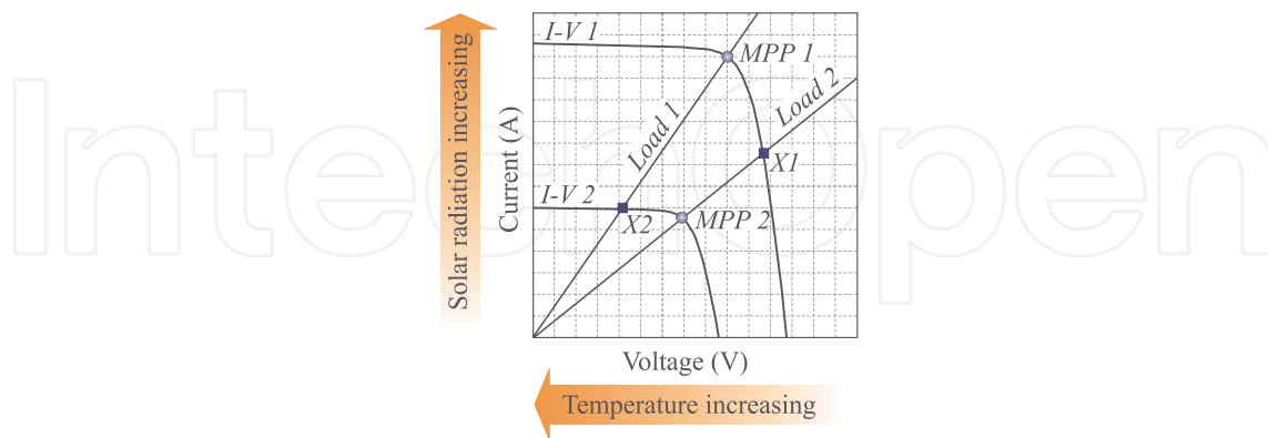
Figure 10. I-V and load curves intersection for defining the PV system operating point.
