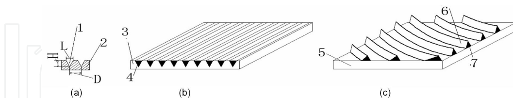
Figure 4. The casting mechanical diagram of rib-like non-smooth structures. (a) the cross-section of rib-like structures. (b) rib-like structures on the rubber plank. (c) paste non-smooth structures to form bionic non-smooth surface on the sand core.
