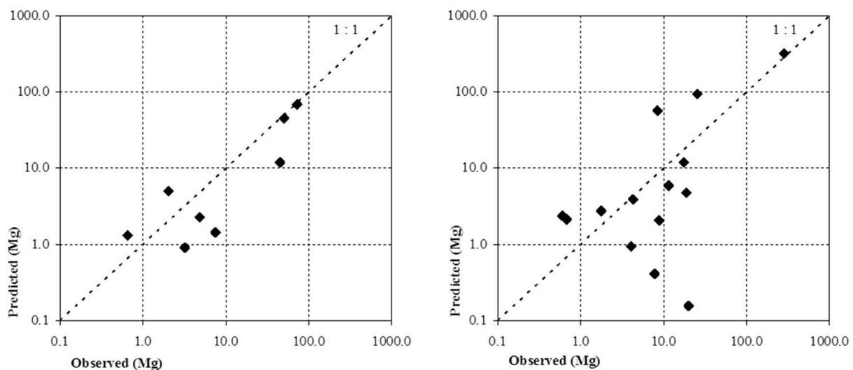
Figure 8. Comparison between observed and simulated sediment yield at event scale for (left) calibration and (right) validation tests at the Cannata watershed.
