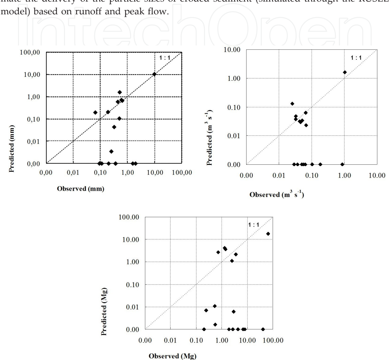
Figure 9. Comparison of 17 observed and simulated (by AnnAGNPS) events in the Ganspoel watershed, for runoff (upper left), peak flow (upper right) and sediment yield (bottom) (values are in logarithmic scale).
