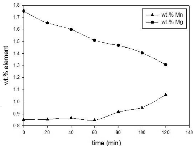
Figure 5. Variation of the concentrations of Mn and Mg, with respect to treatment time, during the metallothermic reduction of \text{Mn}_2\text{O}_3 , for a target Mn concentration of 1 wt. % at constant temperature.
