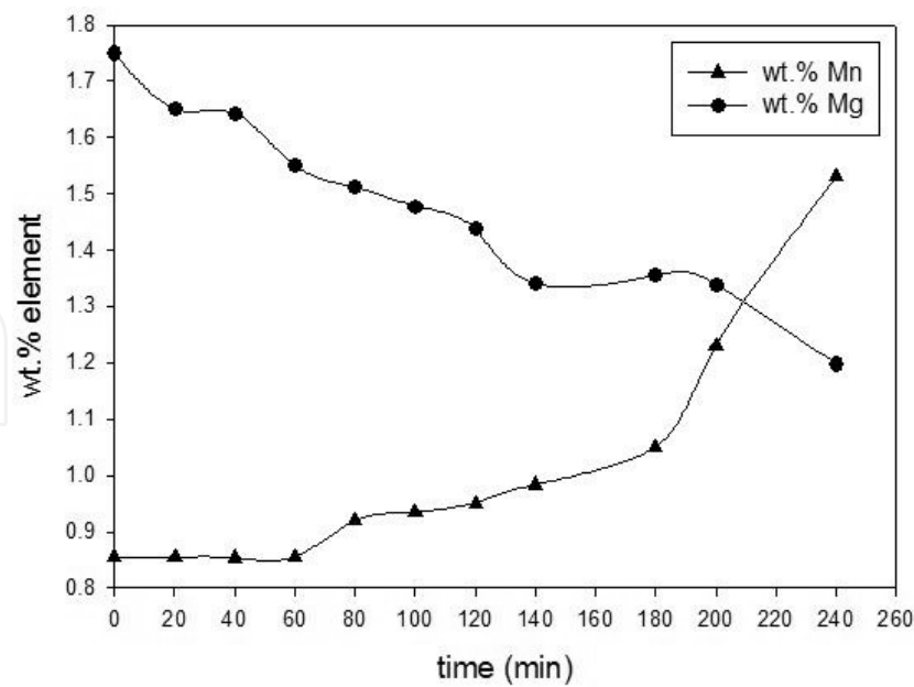
Figure 8. Variation of the concentrations of Mn and Mg, with respect to treatment time, during the metallurgical reduction of \text{Mn}_2\text{O}_3 , for a target Mn concentration of 1.50 wt. % at constant temperature.
