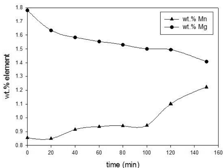
Figure 7. Variation of the concentrations of Mn and Mg, with respect to treatment time, during the metallothermic reduction of \text{Mn}_2\text{O}_3 , for a target Mn concentration of 1.25 wt. % at constant temperature.
