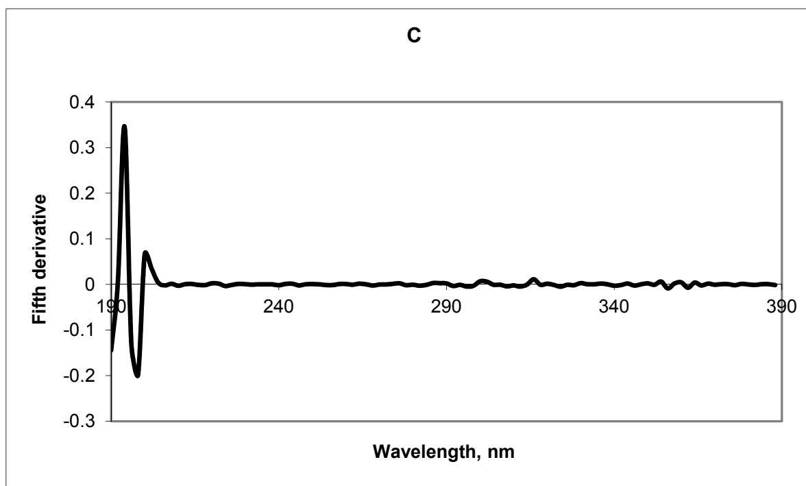
Fig. 2. Zero order (A) and fifth derivative order spectra of ethanol solution of retinol acetate (10 ppm). Spectrum B has been obtained by gradual derivatisation, spectrum C by direct generation of fifth derivative from zero-order spectrum. Apparatus working conditions: Hewlett-Packard HP-8452A diode array spectrophotometer with following working parameters: integration time 1 s, spectral bandwidth 2nm, spectrum scan 0.1 s. Derivative spectra were generated using Savitzky Golay algorithm by PC computer equipped with Excel for Microsoft Windows ( \Delta\lambda=14 nm, fourth polynomial degree).
